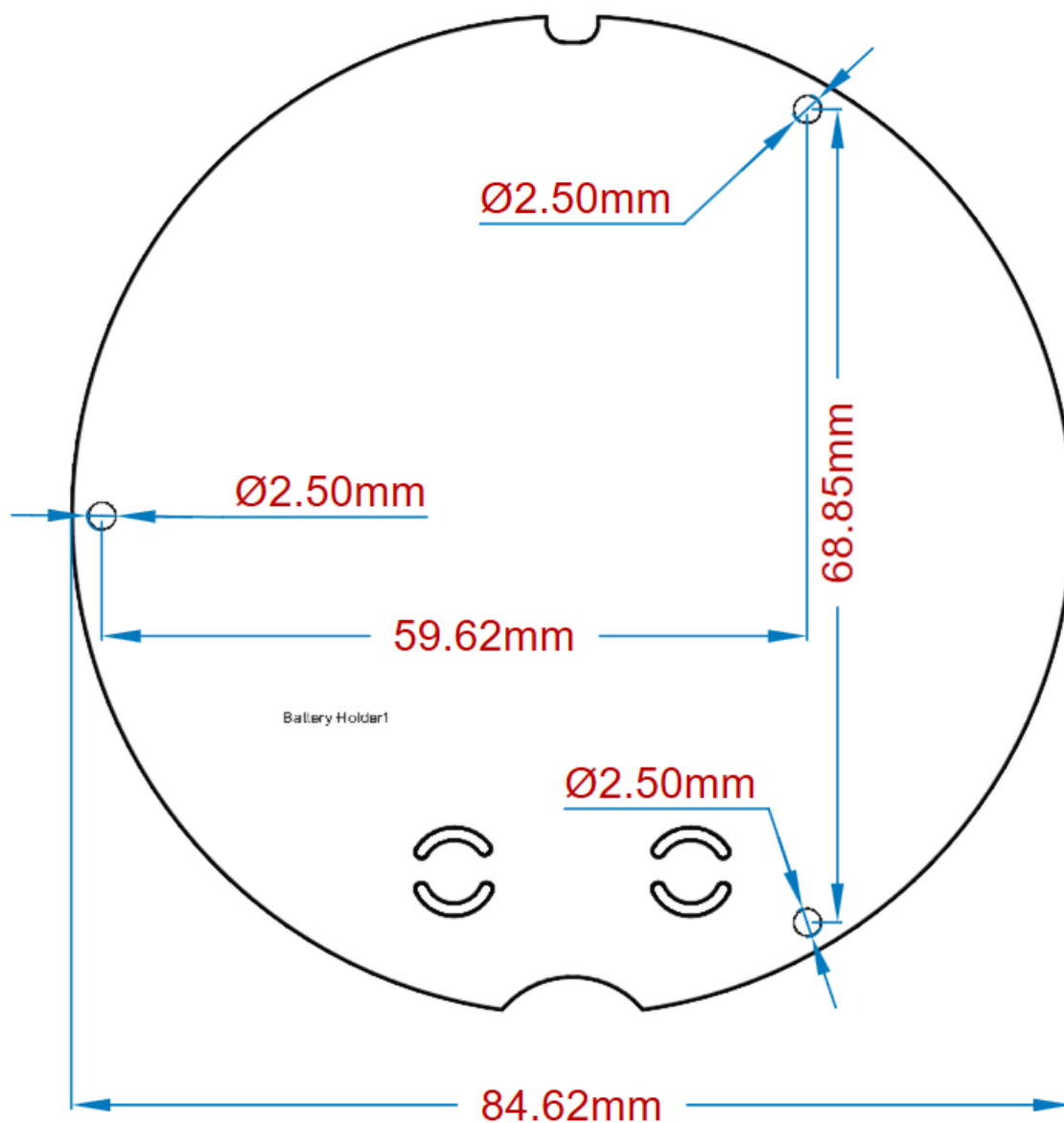
Mechanical view
